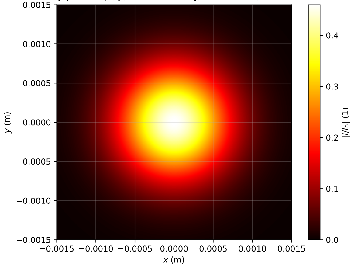
Intensity profile I(x, y, z = 2.548m)/I_0 , P_{in}=0.2P_{cr} , artificial time
